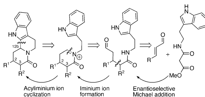
Scheme 1. Retrosynthetic analysis of the indolo[2,3-a]quinolizidine skeleton.
