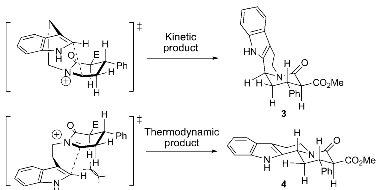
Scheme 3. Kinetic versus thermodynamic product formation in the cyclization of the acyliminium ion.
